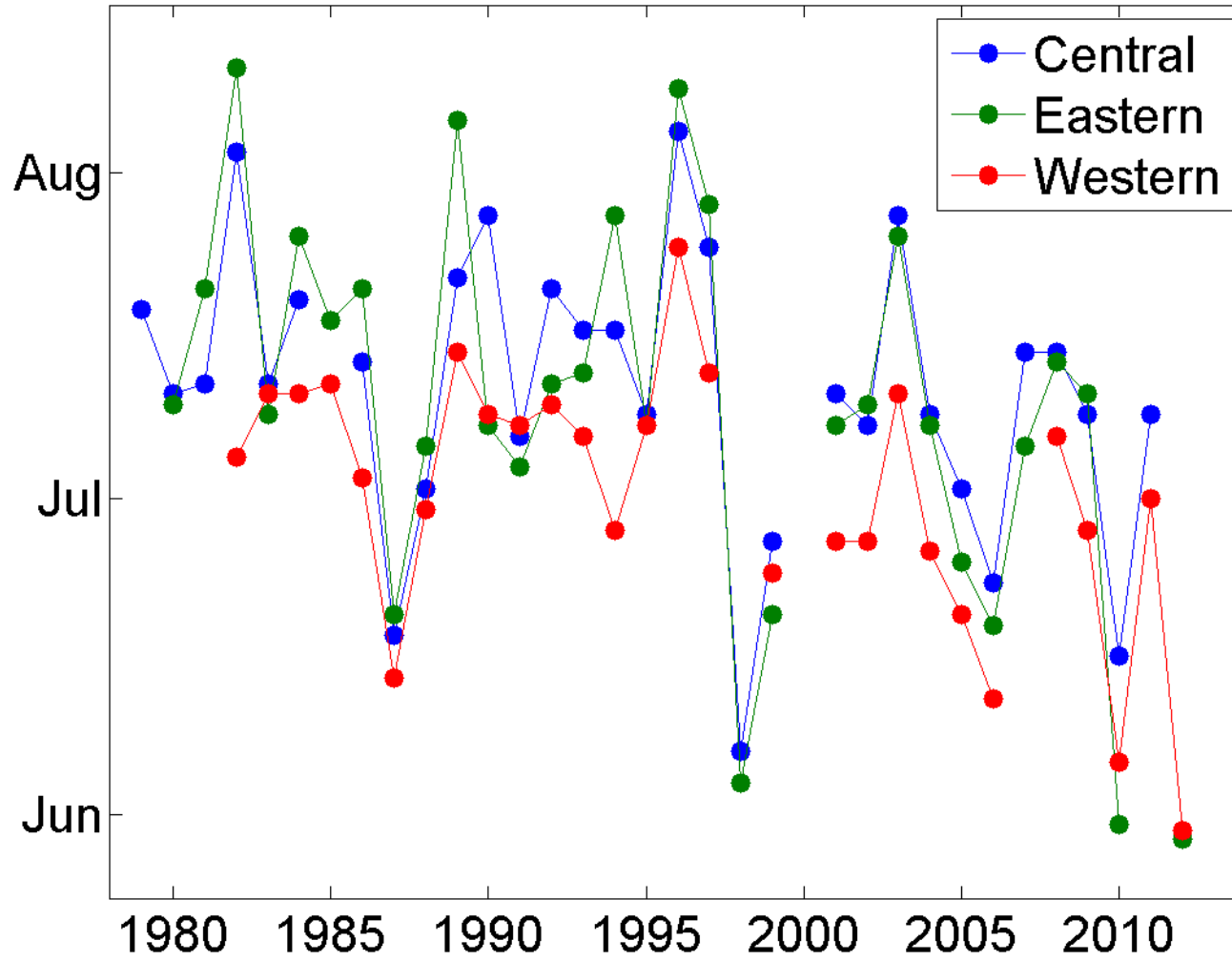
Onset of Lake Superior stratification vs year
